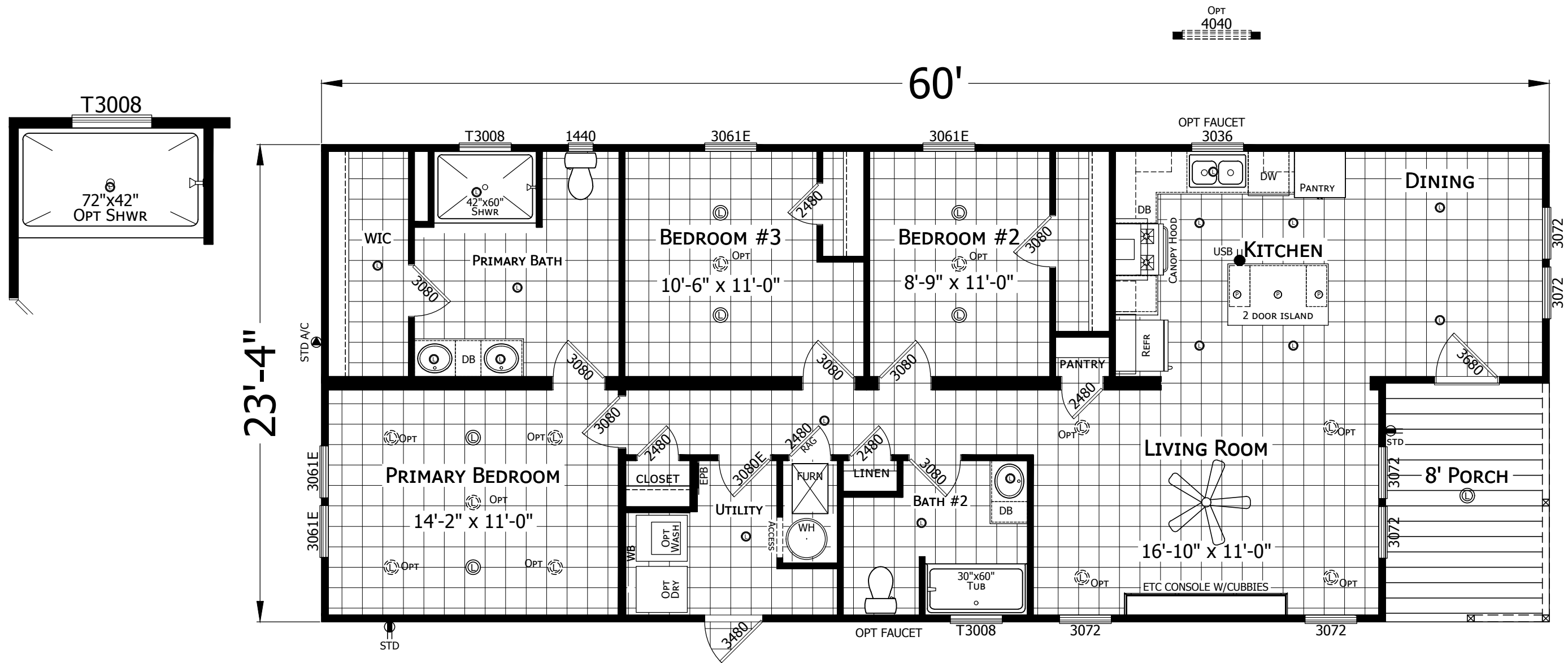
NM2460A-2460H32365 3 BEDROOM 2 BATH 60'-0" x 23'-4" 1400 Sq. Ft. TOTAL
